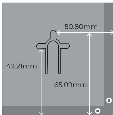
Frame corner screws (Hidden)
